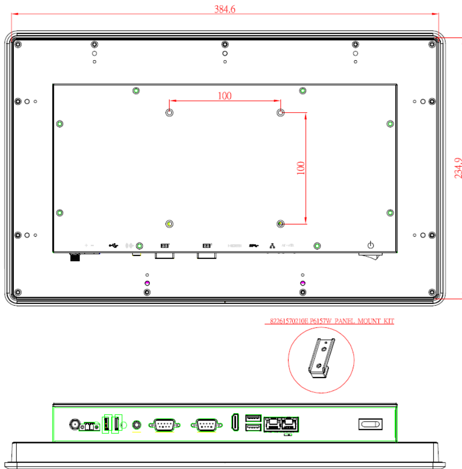
Diagram 1-2 Back outline of the GOT315WL-845-PCT
