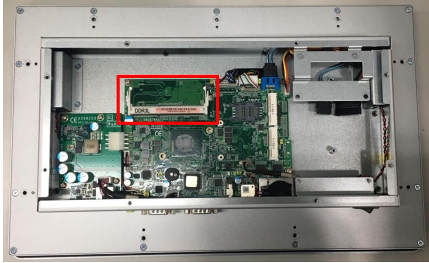
Figure 2-9 DIMM spot
