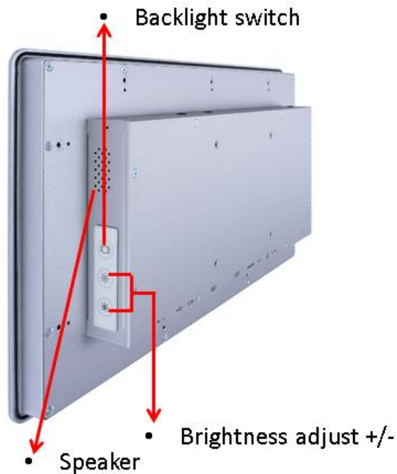
Figure 1-3 Side view of the GOT315WL-845-PCT
