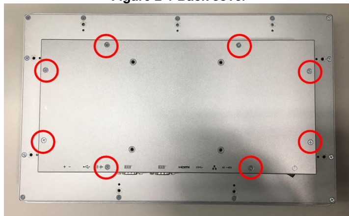
Figure 2-1 Back cover
