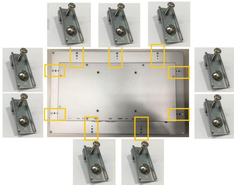
Figure 2-2 Panel mount kit
