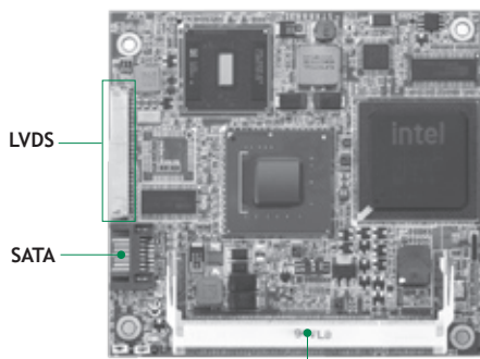
DDR2 SO-DIMM
